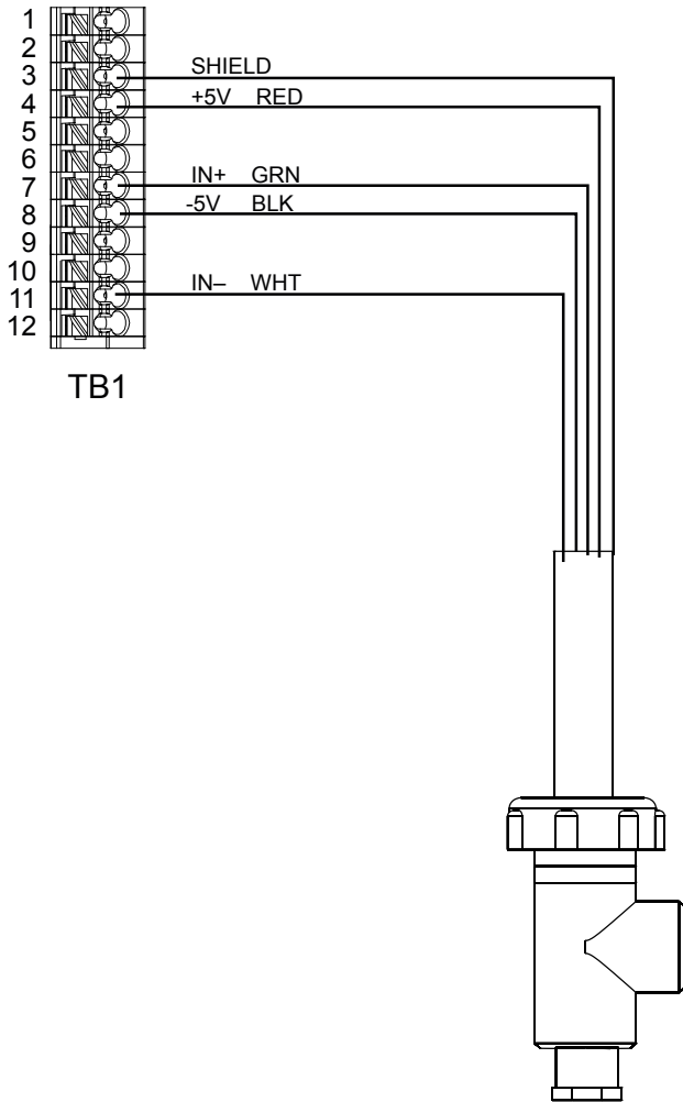
Figure 11 Disinfection/Generic Sensor Input Wiring
