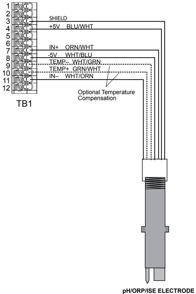
Figure 10 Amplified pH/ORP/ISE Sensor Input Wiring
